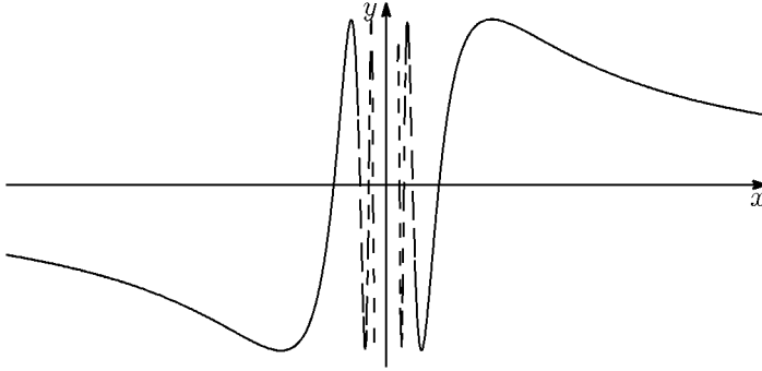
Fig. 1. A non-PostScript plotting of y = \sin(1/x) of a \text{\LaTeX} picture generated by WinTpic
