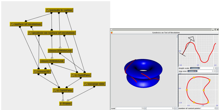
Fig. 3. oorange-network (left) and gui (right) of the application after Step 3
